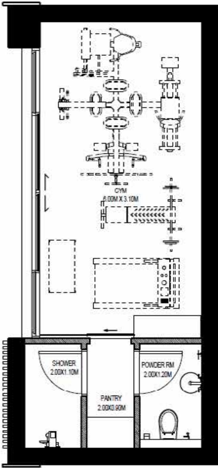
GYM LAYOUT
